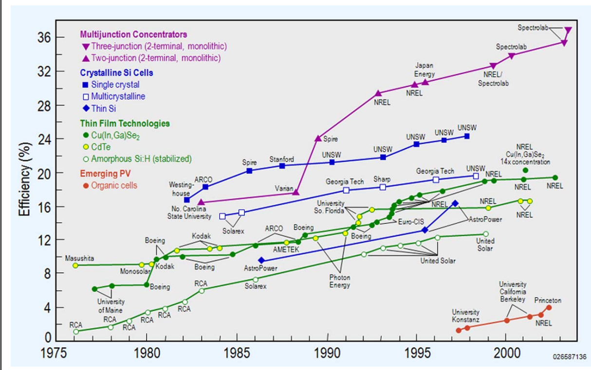
Figure 6: Best Research-Cell Efficiencies
