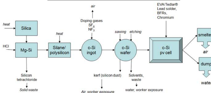
Figure 7: Crystalline Silicon Generic Process Diagram
